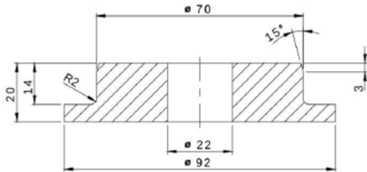
10 GUIDE WASHER MATERIAL: ..... C45 WEIGHT: ..... 0.68 Kgs. SCALE: ..... 1:1
