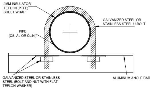
TYPICAL ALUMINUM, CARBON STEEL & COPPER NICKEL PIPE SUPPORT ARRANGEMENT
