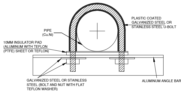
ALTERNATIVE COPPER NICKEL PIPE SUPPORT ARRANGEMENT
